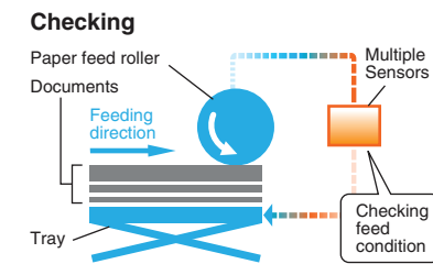
Multiple sensors constantly check the condition of the paper feed and the pressure between the document and the roller.
